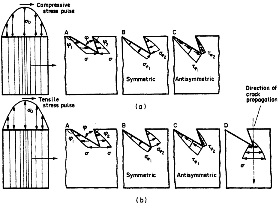
Fig. 6. Diffraction of a stress pulse at an oblique V-notch of initial length depth a_0 : (a) compressive stress pulse; (b) tensile stress pulse, \phi_1 > 90^\circ , \phi_2 < 90^\circ .
