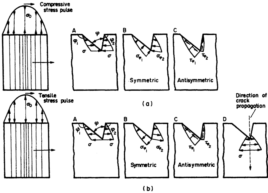
Fig. 5. Diffraction of a stress pulse at an oblique V-notch of initial length depth a_0 : (a) compressive stress pulse; (b) tensile stress pulse, \phi_1 > \phi_2 > 90^\circ .
